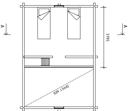
LOFTPLAN 1:100 (A3)
