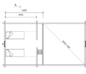
LOFTPLAN 1:100 (A3)
