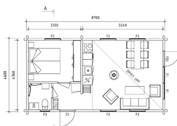
BOTTENPLAN 1:100 (A3)
